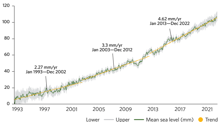
Global mean sea level, 1993–2022 (millimetres)
